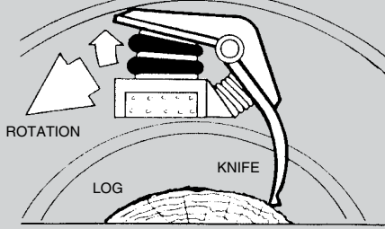
KNIFE SPRING ACTUATOR
