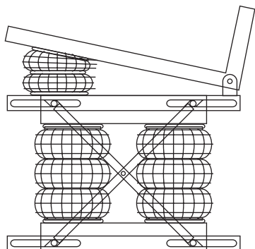
SCISSORS LIFT AND TILT TABLE
