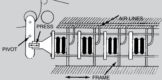
QUICK LOCK DEVICE
